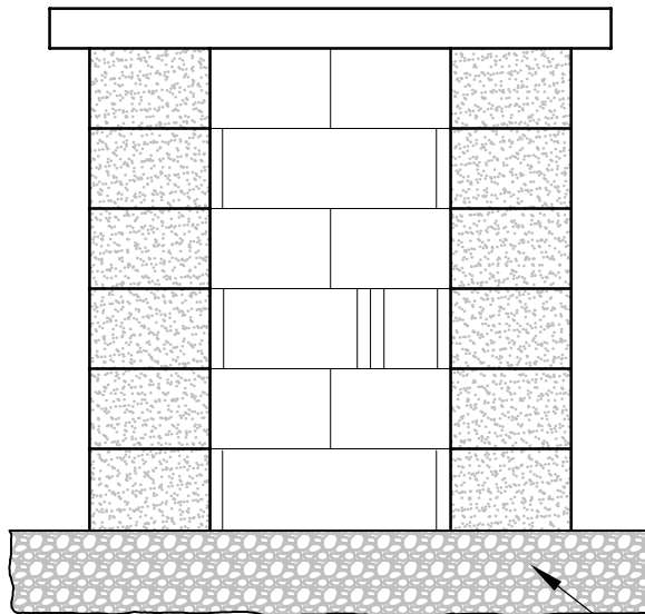
CROSS SECTION (2) (3/4" = 1'-0")
