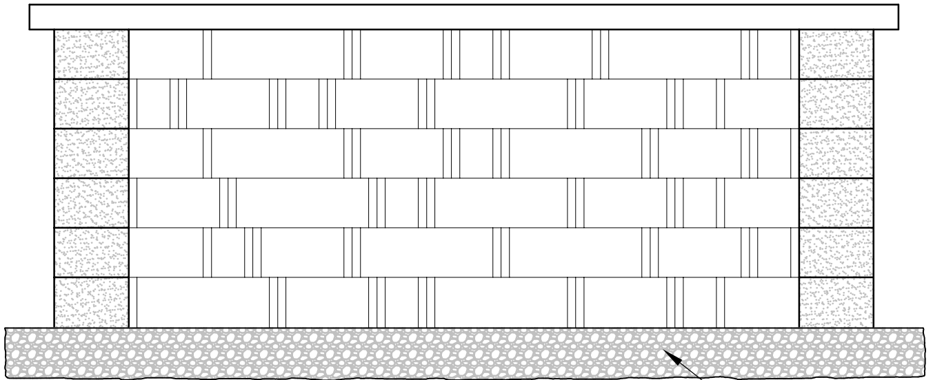
CROSS SECTION (1) (3/4" = 1'-0")
